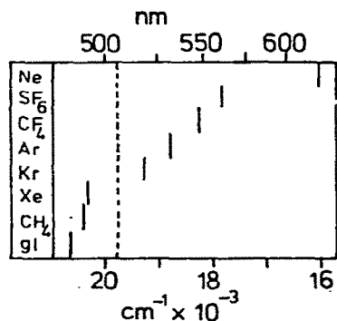
Fig. 13. Dependence of the visible absorption band maximum in \text{Cr}(\text{CO})_5 on matrix material (gl = glass of methylcyclohexane/isopentane). The dotted line is the value found in solution flash photolysis.
