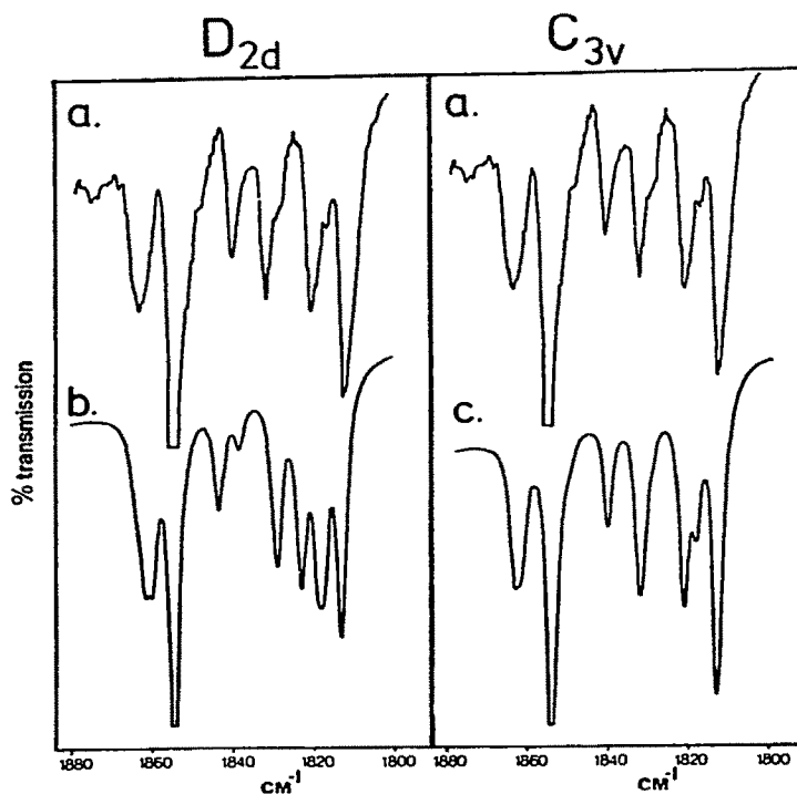
Fig. 8. (a) Observed spectrum in Ar at 12 K; (b) Computer simulated spectrum for the D_{2d} model ( \alpha = 132^\circ ). (c) Computer simulated spectrum for C_{3v} model of \text{Fe}({}^{12}\text{CO})_{4-z}({}^{13}\text{CO})_z ( z = 0-4 ) molecules. (Adapted from ref. 68.)
