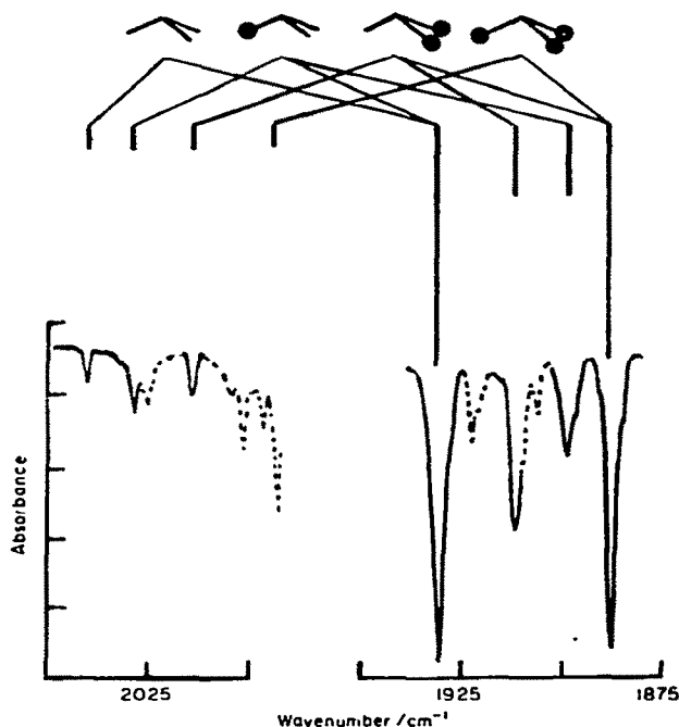
Fig. 5. Observed and calculated (bond angle 109.4^\circ ) IR spectra for a mixture of \text{Fe}(^{12}\text{CO})_{3-z}(^{13}\text{CO})_z ( z = 0-3 ) in a \text{CH}_4 matrix at 20 K. The bands with broken lines are due to \text{Fe}(\text{CO})_{4,5} . The black circles represent ^{13}\text{CO} molecules. (Adapted from ref. 49).
