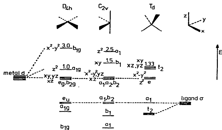
Fig. 12. Molecular orbital diagrams showing ligand \sigma —metal d orbital interactions in terms of the angular overlap model for square planar, octahedral cis divacant and tetrahedral geometries. The numbers showing the destabilization energies of the d -orbitals are in units of \beta_{\sigma} S_{\sigma}^2 . We assume for simplicity here that the stabilization energy of a metal—ligand bonding orbital (mainly ligand located) is the same as the destabilization energy of the corresponding metal—ligand antibonding orbital (mainly metal located). Note the unconventional axis system for the C_{2v} structure. In some descriptions of the AOM the label e_{\sigma} is used in place of \beta_{\sigma} S_{\sigma}^2 .
