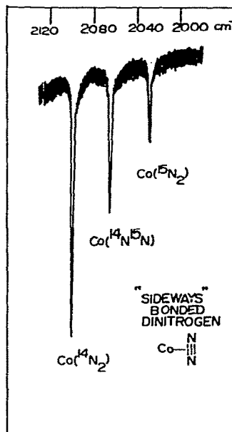
Fig. 9. IR spectrum of \text{Ni}^p\text{N}^q\text{N} ( p, q = 14, 15 ) molecules in a solid \text{N}_2 matrix showing the split central component of the spectrum. (From ref. 87 with permission.)
