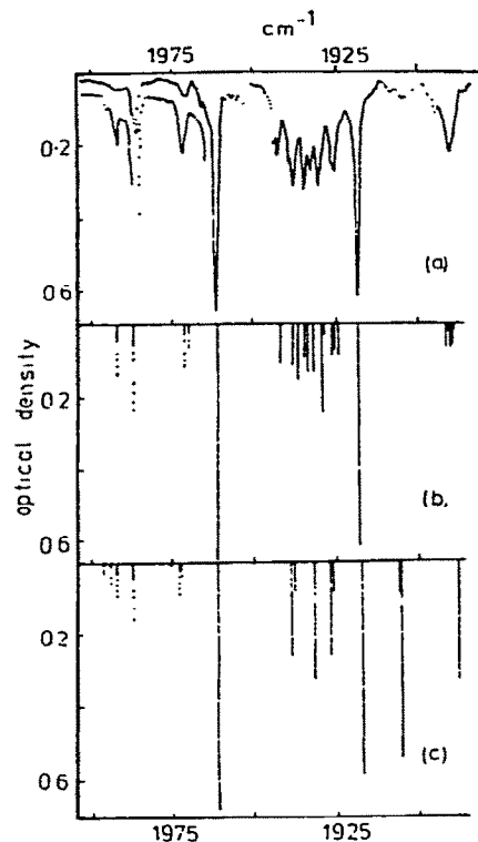
Fig. 6. (a) Observed spectrum of \text{Cr}({}^{12}\text{CO})_{5-z}({}^{13}\text{CO})_z molecules in a \text{CH}_4 matrix at 20 K. (b) Calculated 'stick' spectrum for a C_{4v} model. (c) Calculated 'stick' spectrum for a D_{3h} model. From ref. 53 with permission.
