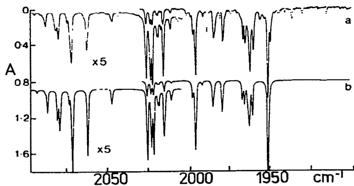
Fig. 7. (a) Observed and (b) computer simulated spectra of \text{Cr}({}^{12}\text{CO})_{5-z}({}^{13}\text{CO})_z\text{CS} ( z = 0-5 ) molecules trapped in a \text{CH}_4 matrix at 20 K. The same half width was used for all the bands in the simulated spectrum which makes the calculated high frequency bands slightly stronger than they should be. The dashed lines in (a) are due to a \text{Cr}(\text{CO})_6 impurity. (From ref. 79 with permission.)
